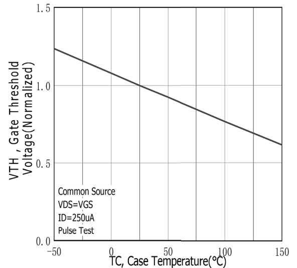
Figure.10 Typical Threshold Voltage vs Case Temperature
